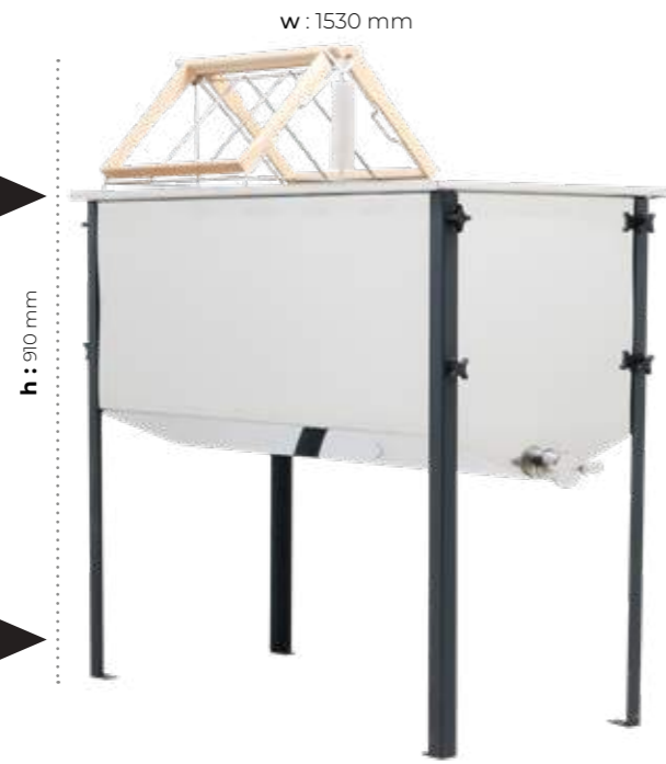
Uncapping Holder AISI 304 Stainless
